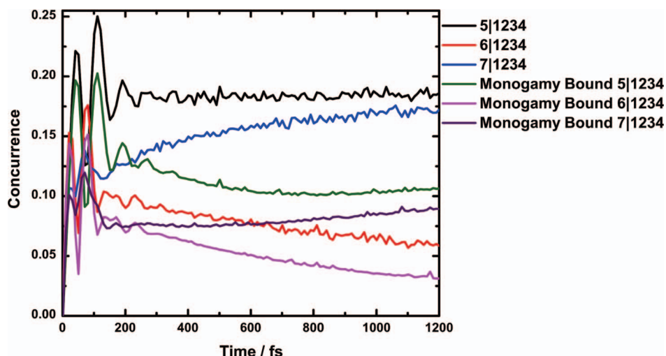
FIG. 10. Evolution of entanglement measures \sqrt{\eta_S} for the subsystems of chromophores 12345, 12346, and 12347 in the FMO complex at cryogenic temperature T = 77 K for site 1 is initially excited. The measures \sqrt{\eta_S} are computed across bipartitions 5|1234, 6|1234, and 7|1234 and the corresponding monogamy bounds are also shown. Site 1, 2, 3, and 4 are sites evolved in the population pathway under this initial condition, and this data indicates that the entanglement of this subset (1234) of chromophores with the other three chromophores is small.
