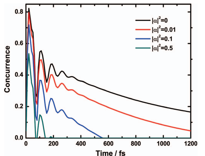
FIG. 17. A comparison of the effects of adding in the two-exciton subspace for different values of |\alpha^2| . The concurrence between sites one and two is plotted for the density matrix in Eq. (21), with |\alpha^2| = 0.5, 0.1, 0.01 .
