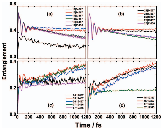
FIG. 15. Entanglement measures \sqrt{\eta_S} for the full FMO system at 77 K with site one initially excited. These four plots show measures \sqrt{\eta_S} computed across all 21 bipartitions of the seven chromophore system into a pair of chromophores and the remaining quintuplet. Any measure that includes either chromophore 1 or chromophore 2 (but not both) on one side of the bipartition exhibits oscillations and the value of the measure is large. Any measure that has both chromophore 1 and 2 on the same side of the bipartition takes lower values and exhibits rapid growth in the first 100 fs, but never exceeds 0.5 in value.
