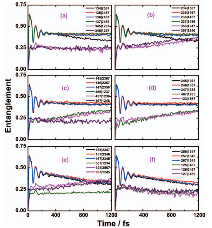
FIG. 16. Entanglement measures \sqrt{\eta_S} for the full FMO system at 77 K with site one initially excited. These six plots show measures \sqrt{\eta_S} computed across all 35 bipartitions of the seven chromophore system into three of chromophores and the remaining four. Any measure that includes either chromophore 1 or chromophore 2 (but not both) on one side of the bipartition exhibits oscillations and the value of the measure is large. Any measure that has both chromophore 1 and 2 on the same side of the bipartition takes lower values and exhibits rapid growth in the first 100 fs, but never exceeds 0.5 in value.
